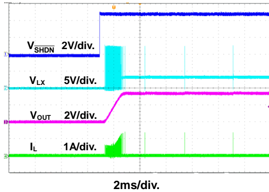
Figure 16. Startup Through \overline{SHDN} Waveform
